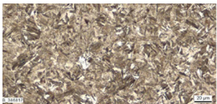
Tempered state, oil cooled 500:1
